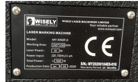
Nameplate Marking
